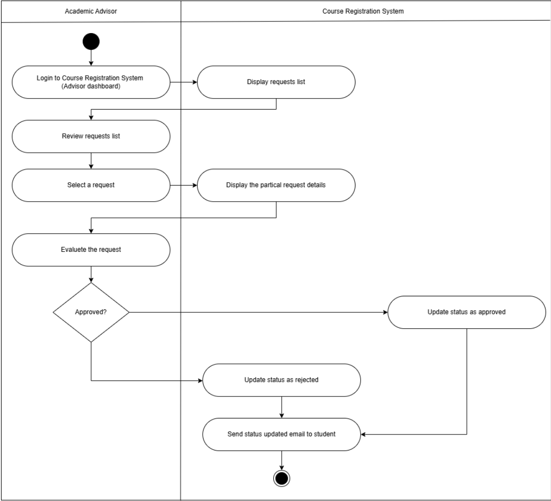
Figure 4.31 Activity Diagram for Add/Drop Approval Workflow
