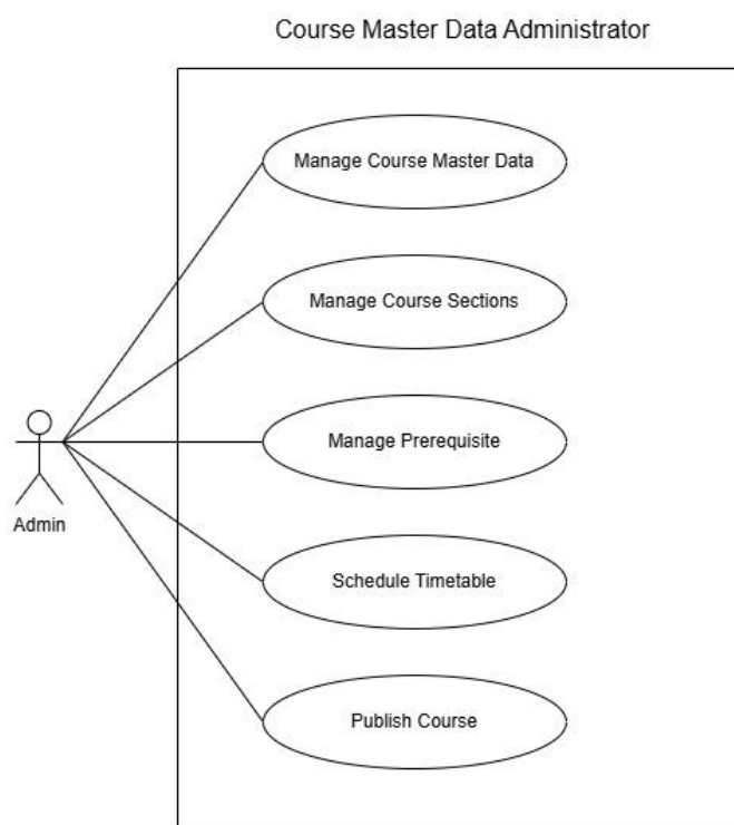
Figure 4.37 Use Case Diagram for Course Master Data Administrator
