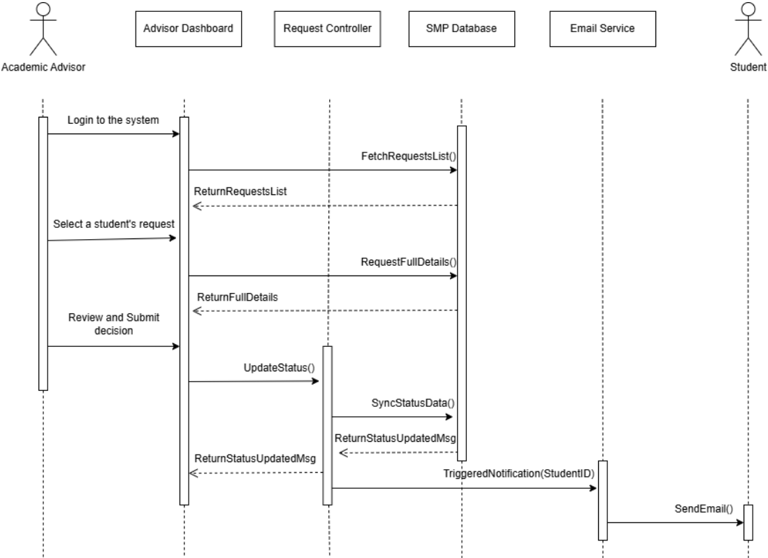
Figure 4.32 Sequence Diagram for Add/Drop Approval Workflow
