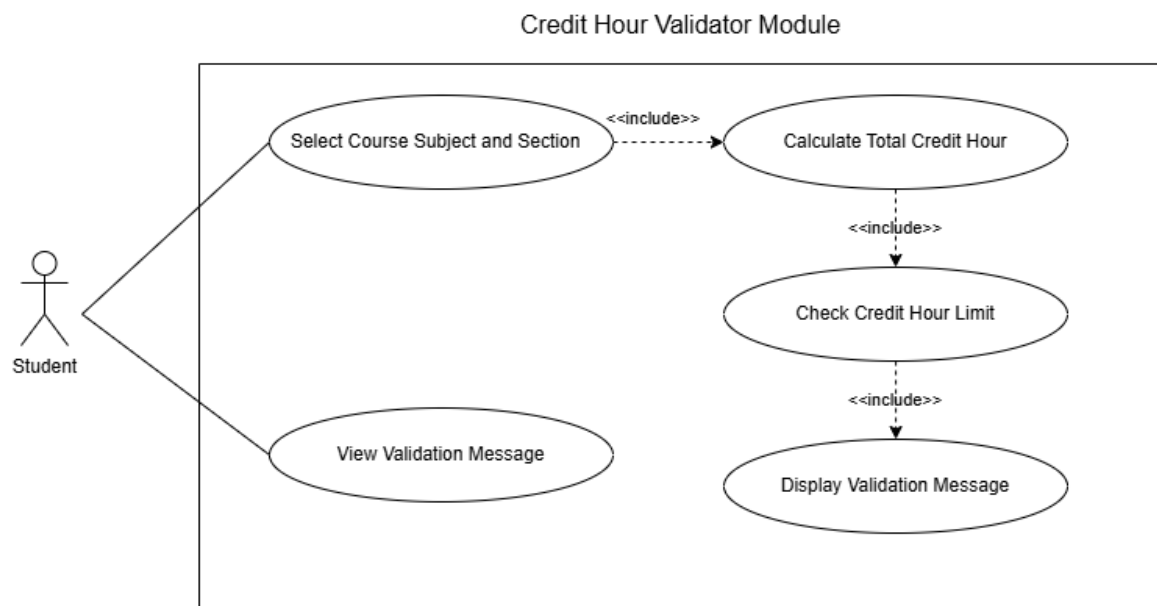
Figure 4.24 Use Case diagram for Credit Hour Validator Module
