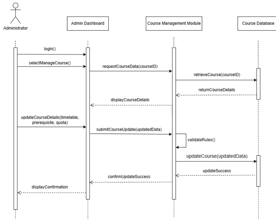
Figure 4.39 Sequence Diagram for Sub-Module Course Master Data Administrator
