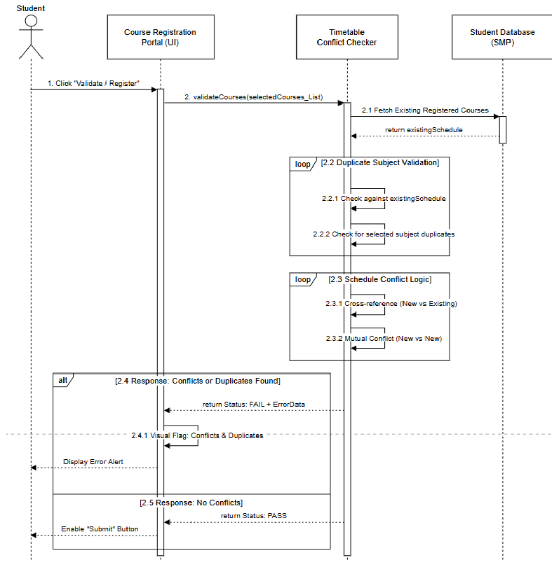
Figure 4.18 Sequence Diagram for Timetable Conflict Checker Module
