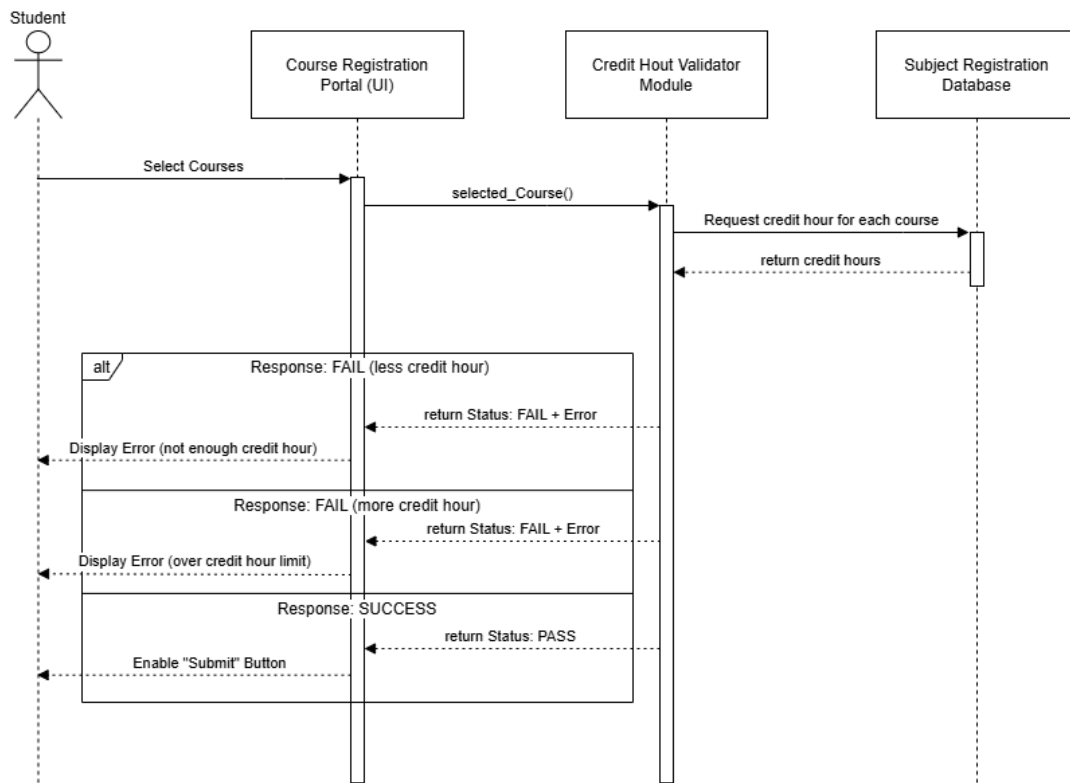
Figure 4.26 Sequence diagram for Credit Hours Validator Module
