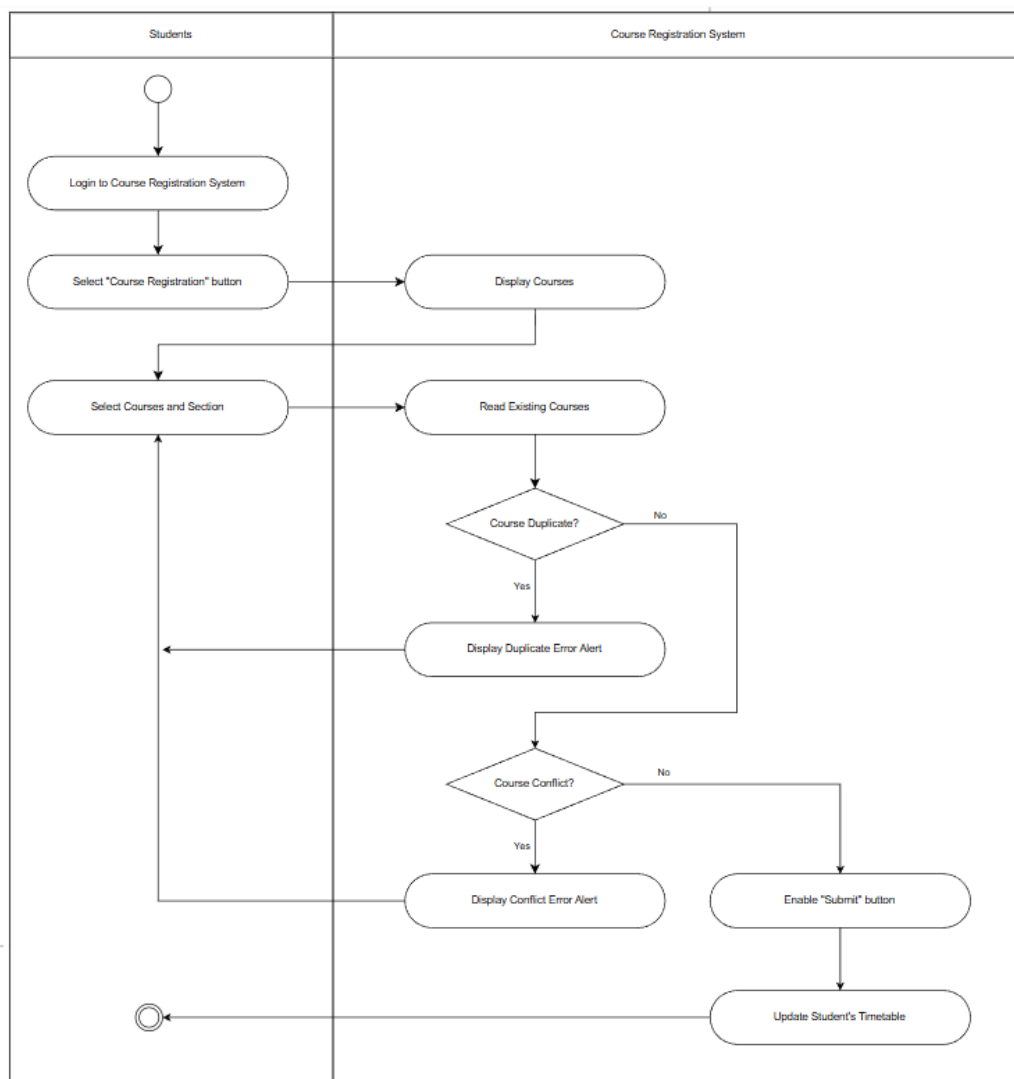
Figure 4.19 Activity Diagram for Timetable Conflict Checker Module
