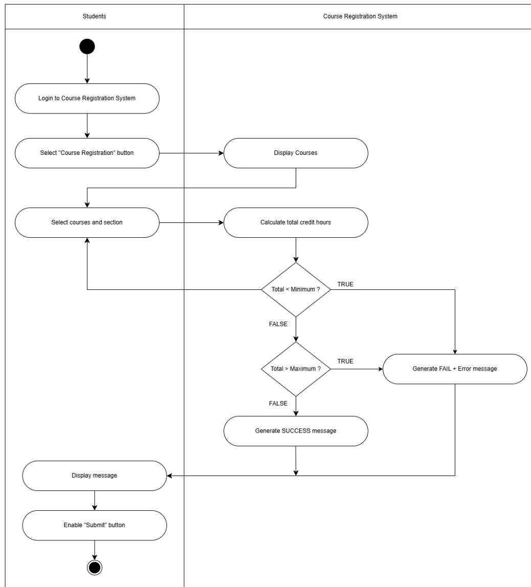
Figure 4.25 Activity diagram for Credit Hours Validator Module
