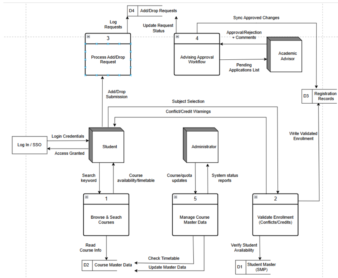
Figure 4.2 Current System Diagram
