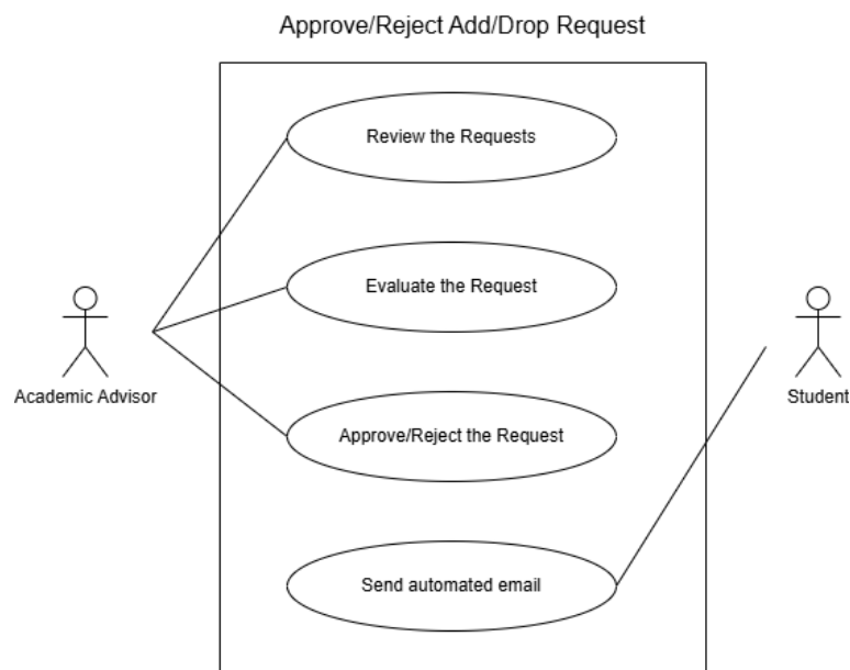
Figure 4.30 Use Case Diagram for Add/Drop Approval Workflow
