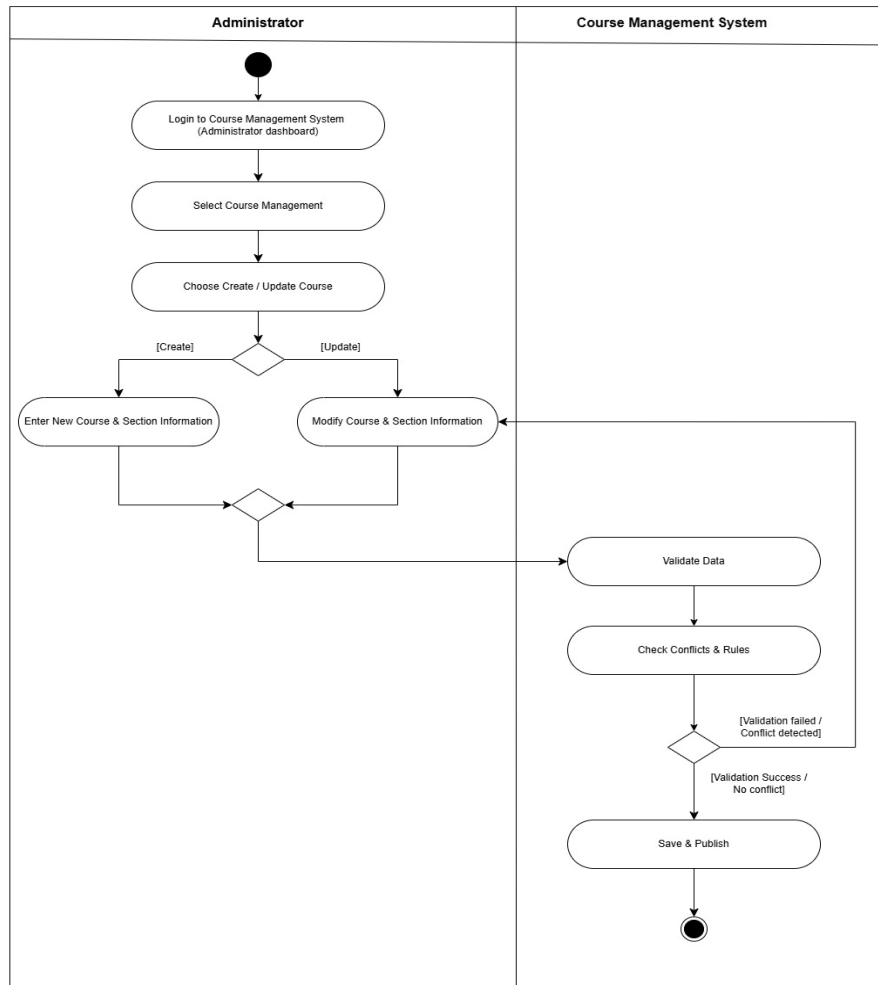
Figure 4.38 Activity Diagram for Sub-Module Course Master Data Administrator
