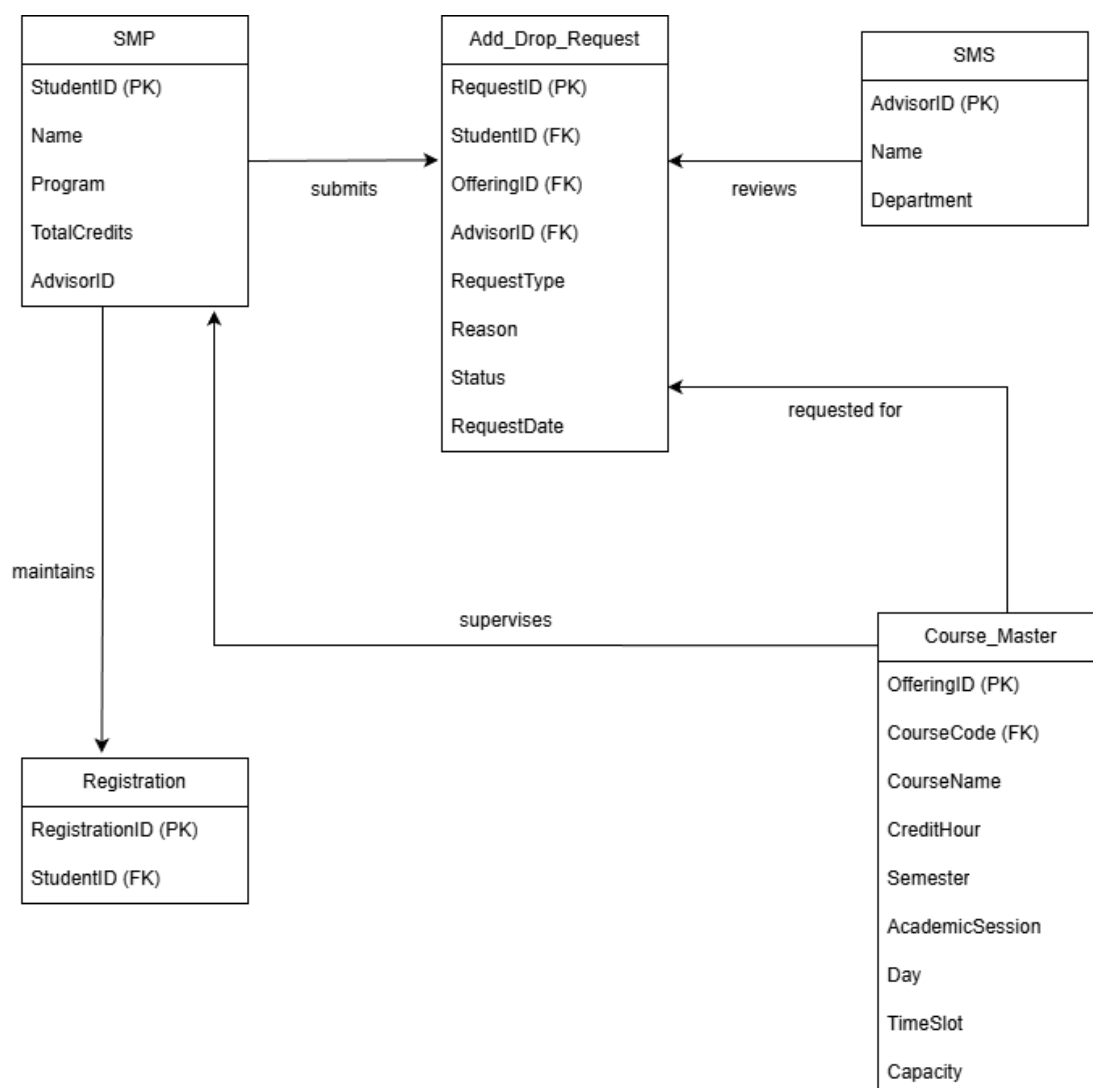
Figure 4.6 ERD Diagram for the Subject Registration Enhancement Module
