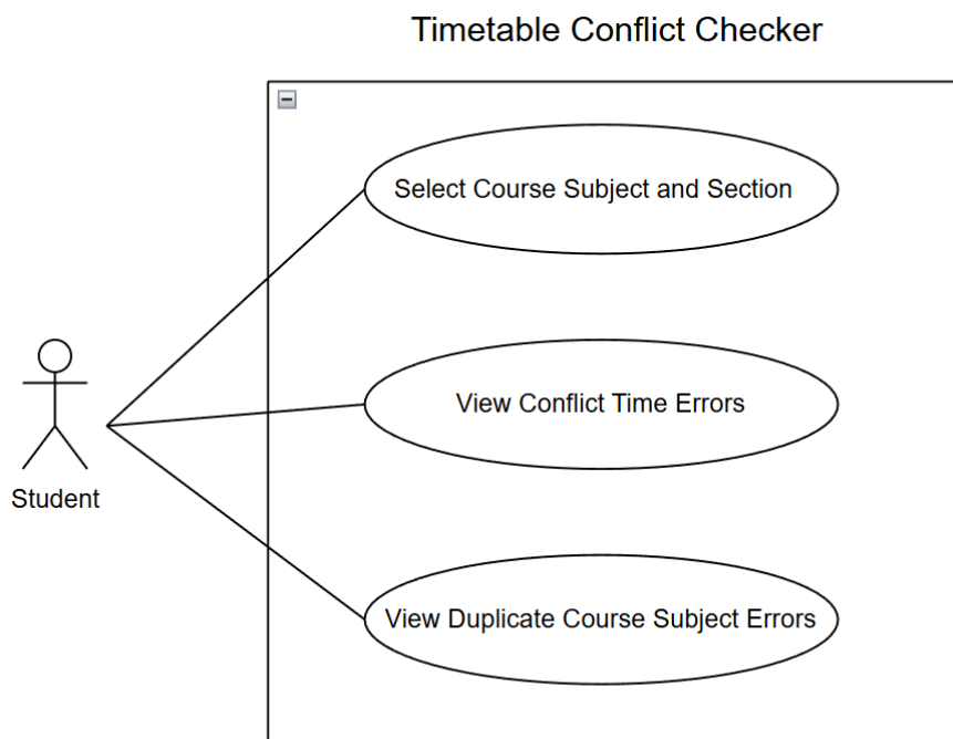
Figure 4.17 Use Case Diagram for Timetable Conflict Checker Module
