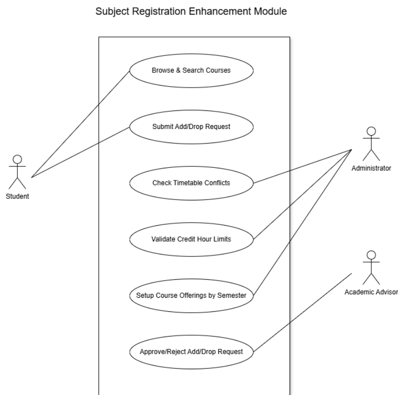
Figure 4.5 Use Case Diagram for the Subject Registration Enhancement Module
